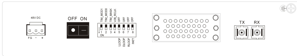
Rear Panel of MODEL7304/DC
