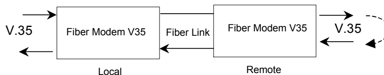
Remote Loopback
